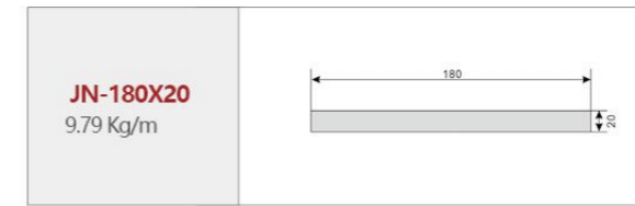
铝大梁, 导电铜座 Aluminum beam, conductive copper base
